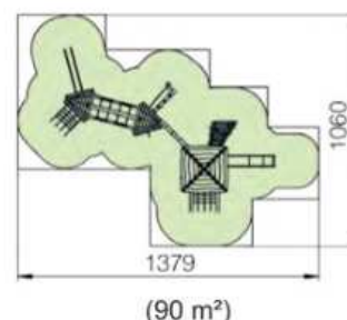
RO550 (maxi magic tower with roof, with suspension loops) RO552 (maxi magic tower with roof, with balance trail)
