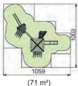
RO540 (magic tower combination with roof, with suspension-loops)
